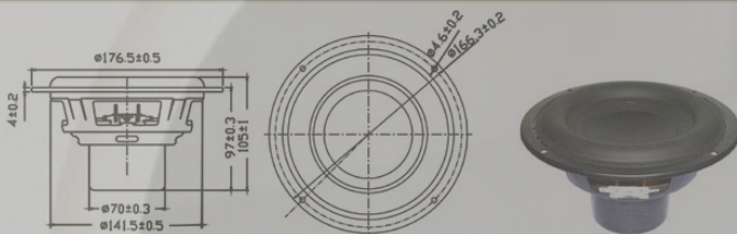
6.5" PAPER SUBWOOFER
